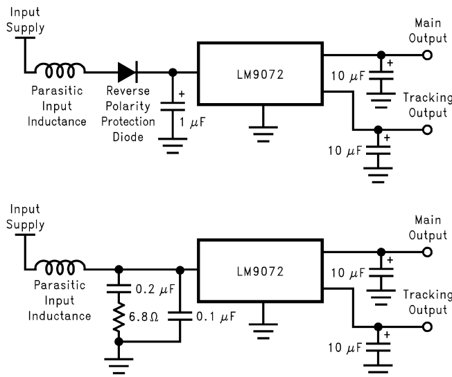
Figure 21. Input Bypassing
